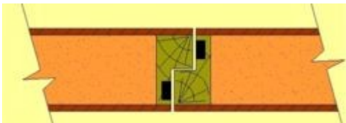
Timber Rebated Meeting Stiles
