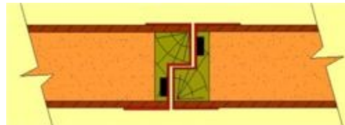
Timber Rebated Meeting Stiles With Metal Capping
