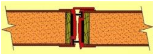
Aluminium Single or Double T-Bar Meeting Stiles
