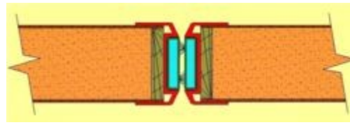
Aluminium Bullnose Meeting Stiles
